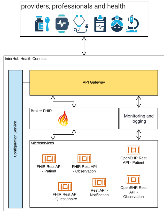
Fig. 5. Interoperability Hub GIRLS (source: author, 2019).
