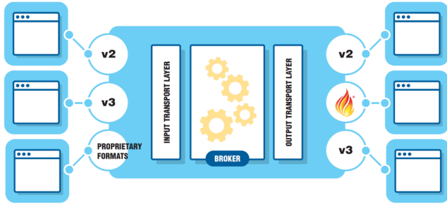
Fig. 3. Figure 3 - FHIR Broker: converts different data formats into FHIR format (source: Interopera, 2018).
