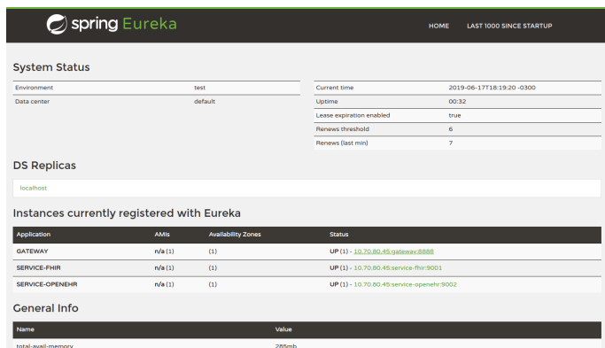
Fig. 7. Running GIRLS Prototype (source: author, 2019).
