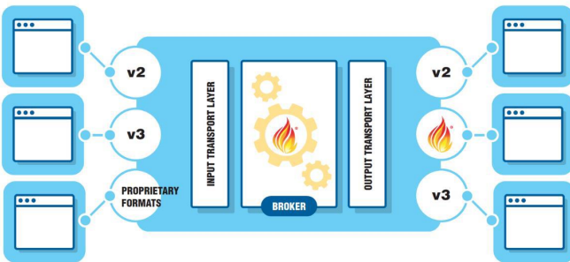
Fig. 4. FHIR as an Integration Hub (source: Interopera, 2018)
